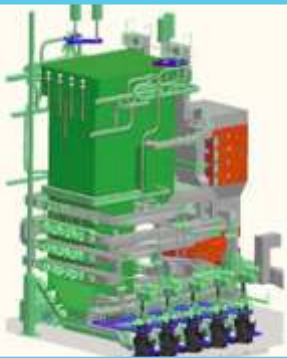
SUBCRITICAL BOILER
